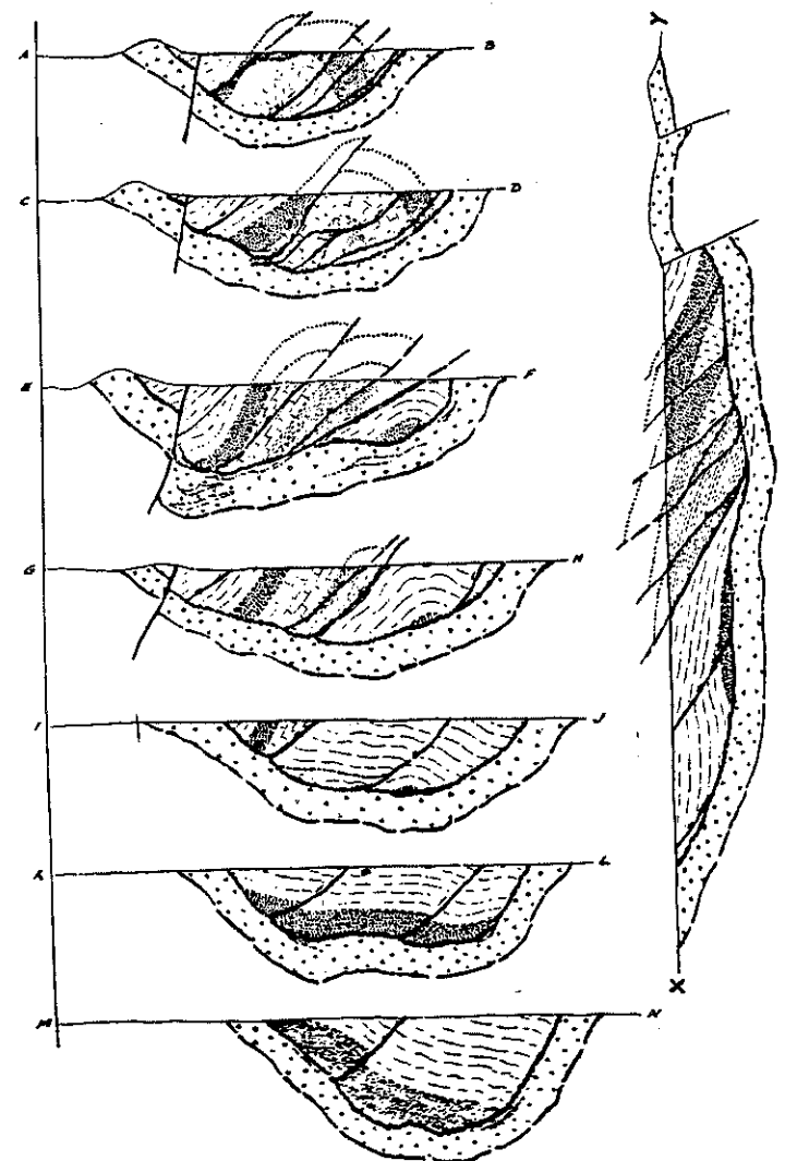
Fig. 32: Geological sections through Alaska Mine (after Jacobsen, 1964). The section lines are shown in Fig. 31.
