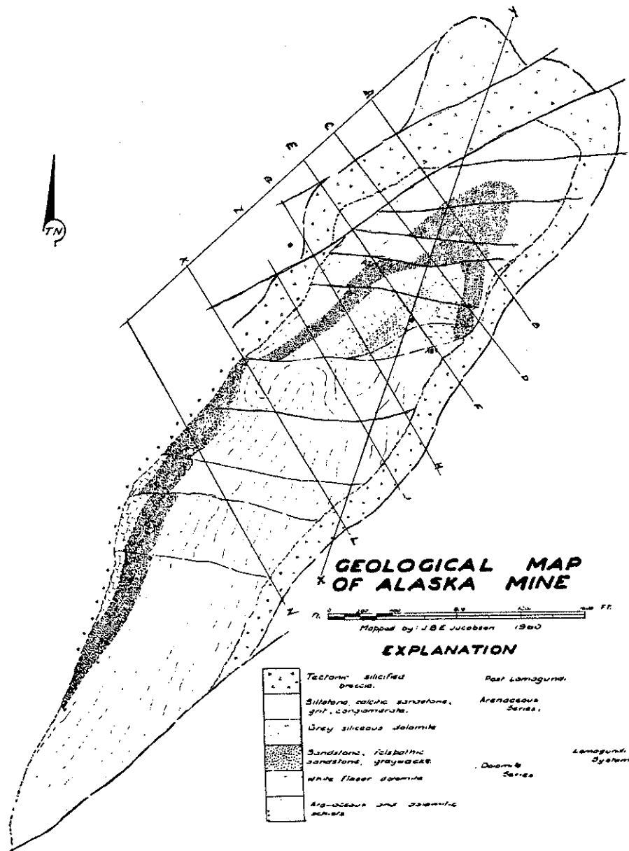
Figure 31: Geological map of Alaska Mine (after Jacobsen, 1964).
